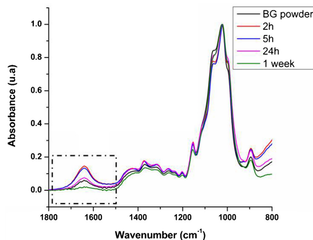
Fig. 3. FTIR spectra of \beta -D-glucan freeze-dried samples obtained from a 1 wt.% \beta -D-glucan solution heat treated at 85 °C for 2, 5, and 24 h, and 1 week, as well as for the pristine sample.
